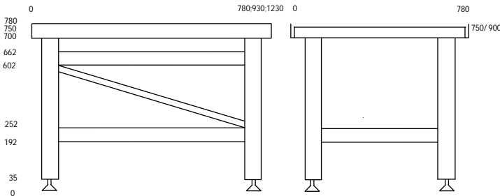
Dimensions mm's
